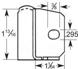
No. 48 Bolted For Outside Angle Iron
